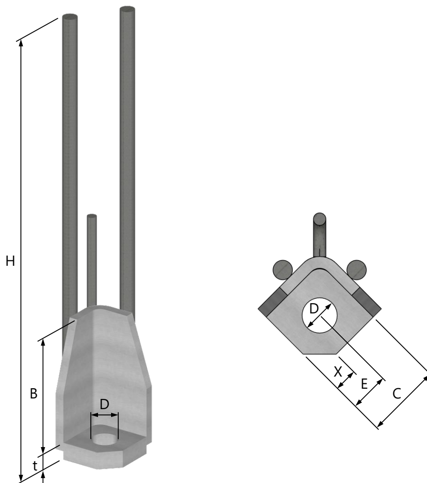
Figure 1. Dimension markings of RPK-N3 column shoes
